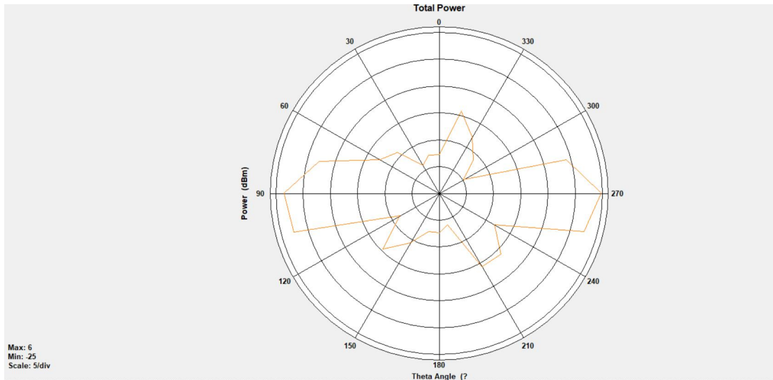
2D Radiation Pattern at 3700MHz
